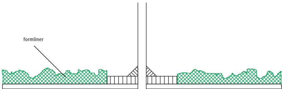
SMOOTH FRAME WITH CHAMFER HIGH IN CONCRETE
