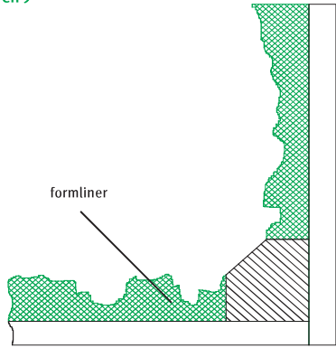
COVE WITH CHAMFER, DEEP IN CONCRETE
