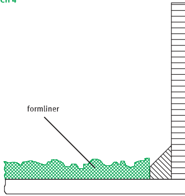
CHAMFERED COVE, HIGH IN CONCRETE
