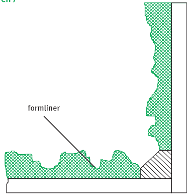
COVE WITH CHAMFER, HIGH IN CONCRETE
