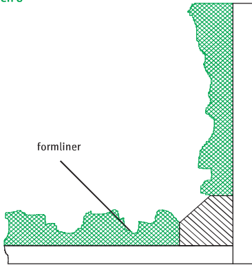
COVE WITH CHAMFER, MIDDLE IN CONCRETE
